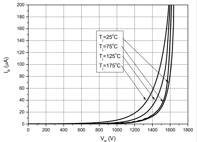
Figure 2. Reverse Characteristics
