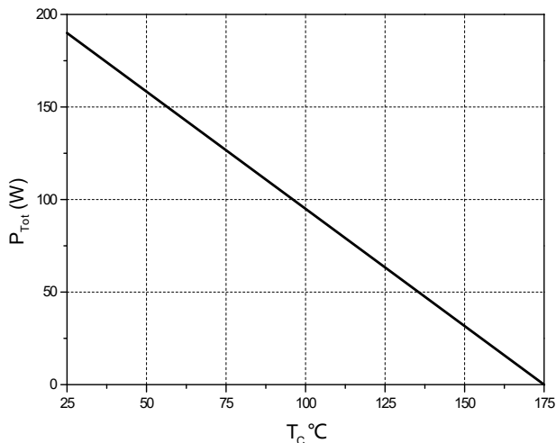
Figure 6. Power Derating
