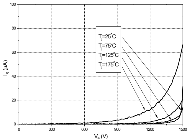
Figure 2. Reverse Characteristics
