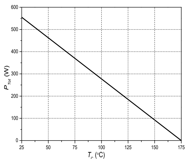
Figure 6. Power Derating
