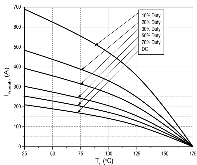
Figure 7. Current Derating
