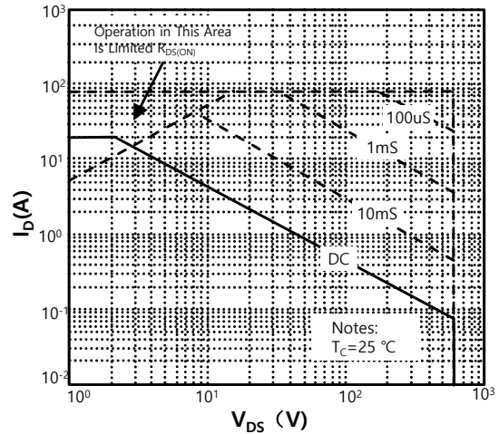
Figure 9-1. Maximum Safe Operating Area (SLF60R190S2)
